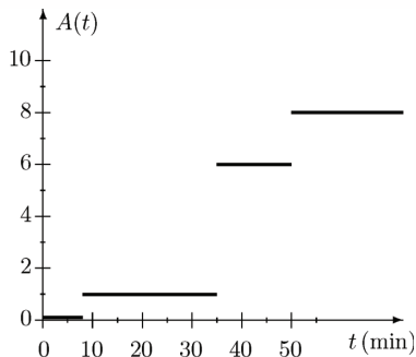
Figure 3: Counting processes in Example 3.2
