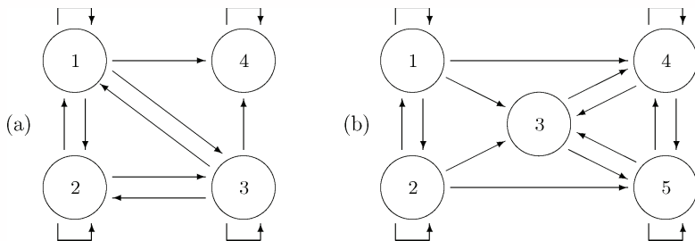
Figure 2: Absorbing states and absorbing zones
