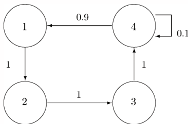
Figure 1: Transition diagram for the regular Markov chain in Example 2.22
