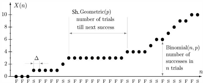
Figure 4: Binomial process sample path ( S = success, F = failure)
