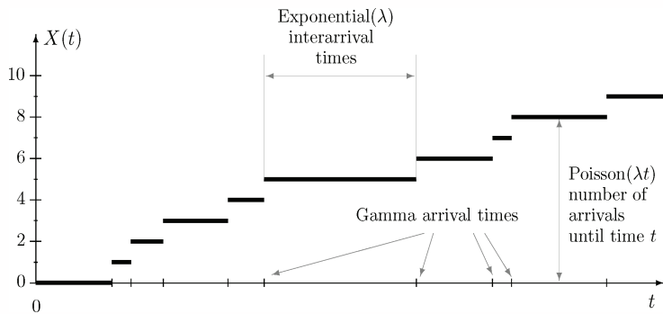
Figure 2: Poisson process sample path
